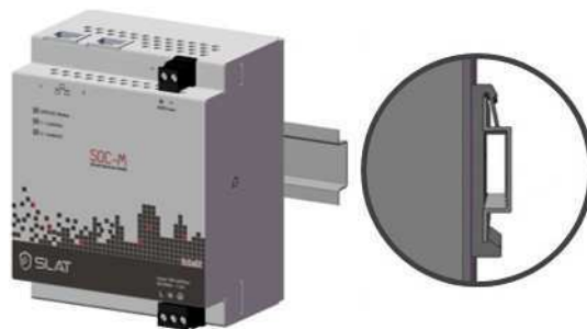
Figure 8.1: Position sur rail DIN
