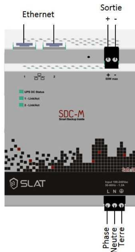
Figure 8.2: Câblage
