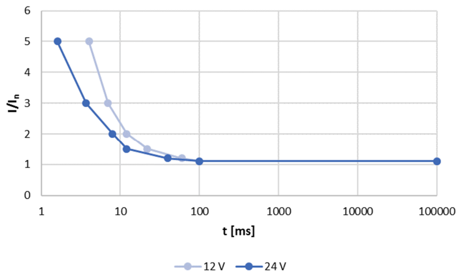
Figure 12.4: Courbe de surcharge admissible
