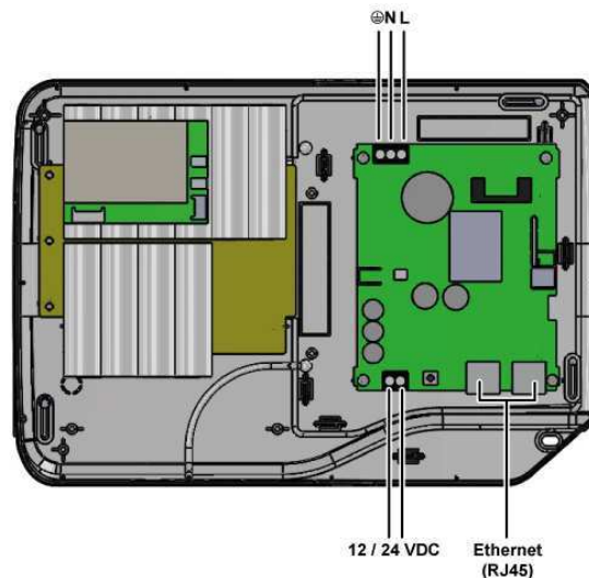
Figure 8.6: Câblage
