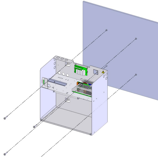
C85 – Abm.: 408x408x224 mm – IP31
